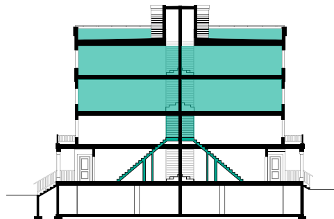
SITE SECTION
