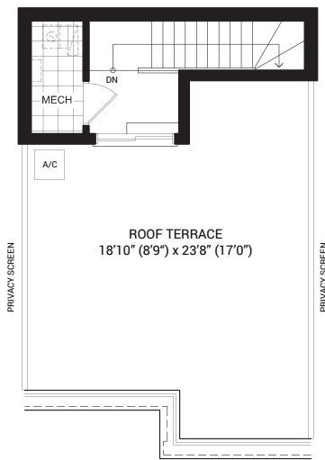
MODEL 2B ROOF TERRACE LEVEL
