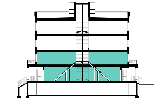
SITE SECTION
